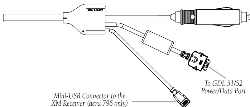
GDL 51/52 Power/Data Cable to Aera 795/796
