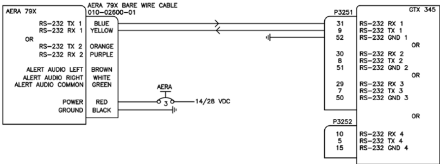
GTX 345 Serial Interface to Aera 795/796
